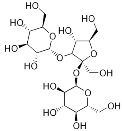
structural formula of honey
